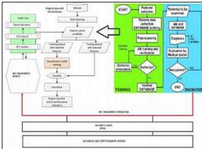
Fig 1: Proposed Architecture
